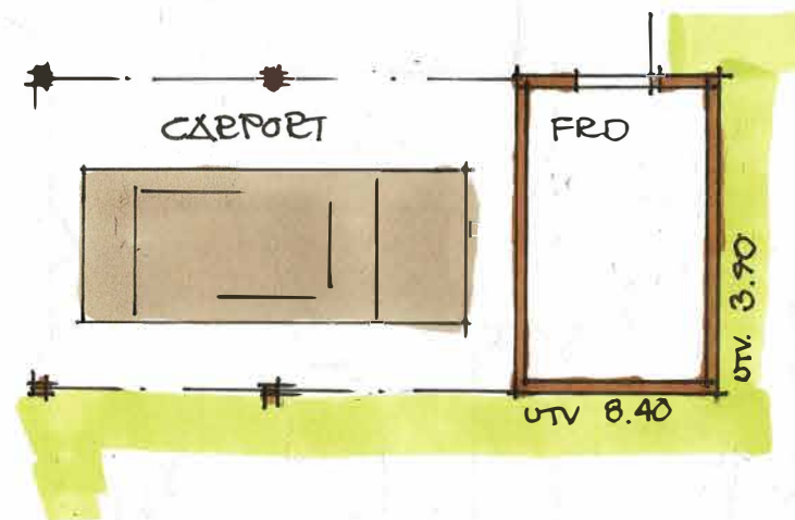
ENTREPLAN. BOA 90,0m 2 (INV. AREA) BYA 149,5m 2 + 32,8m 2
